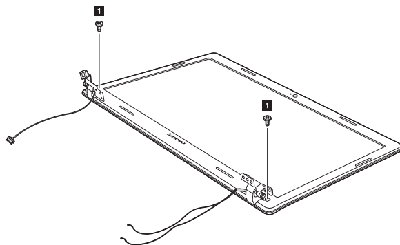
Figure 16. Removal steps of LCD front bezel
