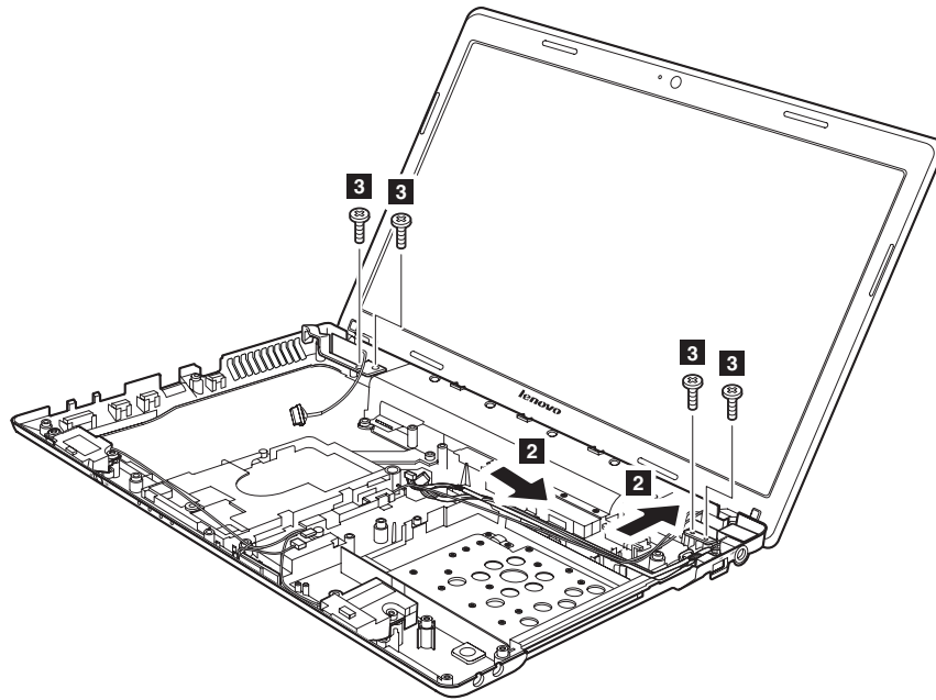
Figure 14. Removal steps of LCD unit (continued)
